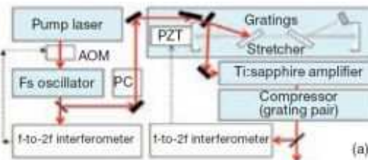
Fig. 1. Schematic of the laser system.
