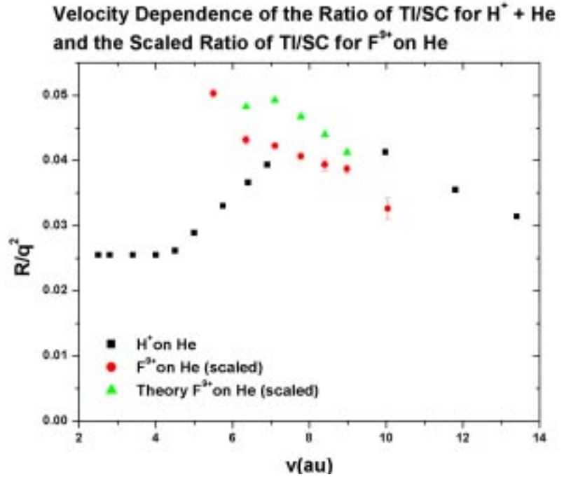
Fig. 1 Transfer Ionization to Single Capture Ratio
